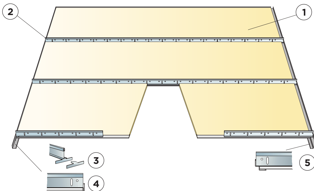
Installation diagram (M17) for Focus D/A in corridor
